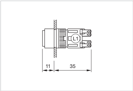
Dimensions [mm] L1 = Solder terminal 2.8 x 0.5 mm
