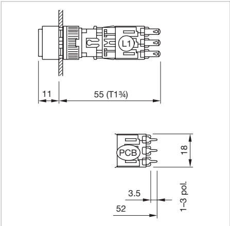
Dimensions [mm] L1 = Solder terminal 2.8 x 0.5 mm, PCB = Print terminal
