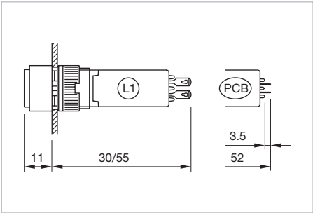
Dimensions [mm] L1 = Solder terminal 2.8 x 0.5 mm, PCB = Print terminal
